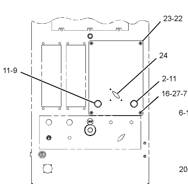
FRONT VIEW (CONTROL PANEL)
